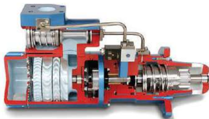
Pneumatic Starters
